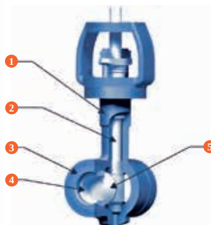
1 Body 2 Shaft 3 Retainer 4 Seat 5 Plug
